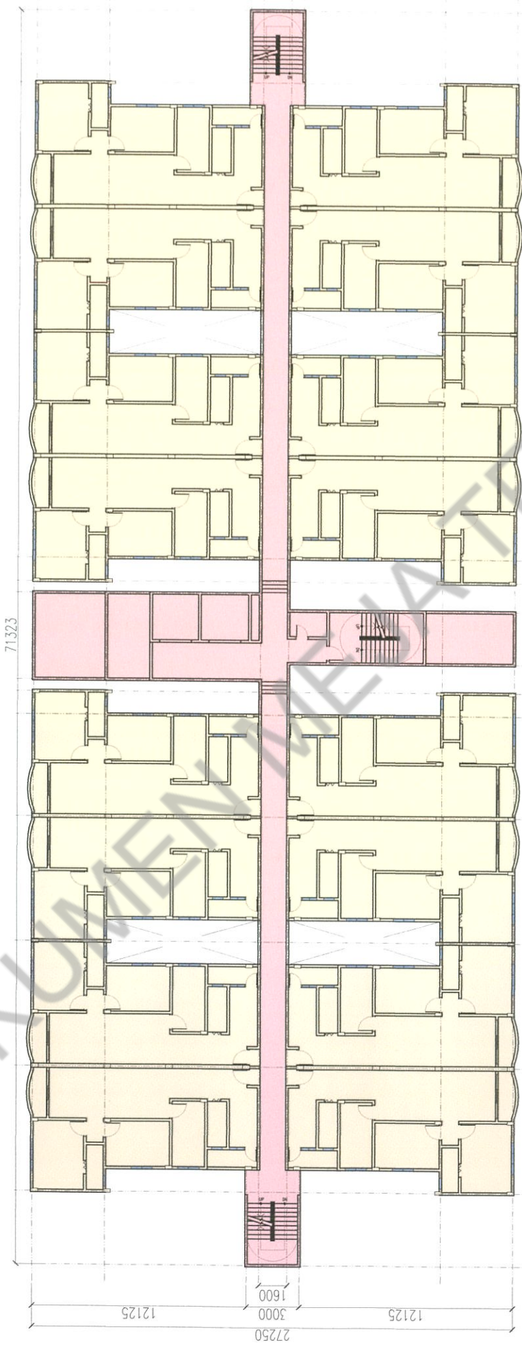
1ST. FL. TO 9TH. FL. PLAN scale : 1:200
