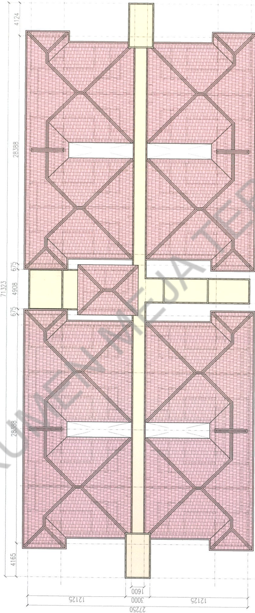
ROOF PLAN SCALE : 1:200
