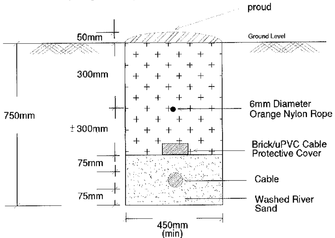
Figure 1: Cable Laid Direct In Ground
