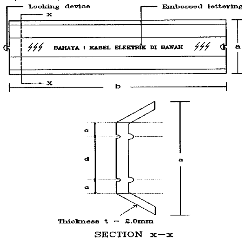
Figure 2: uPVC Cable Protective Cover
