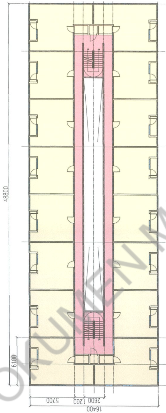
1ST. FL. TO 4TH. FL. PLAN (BLOCK A) scale : 1:100
