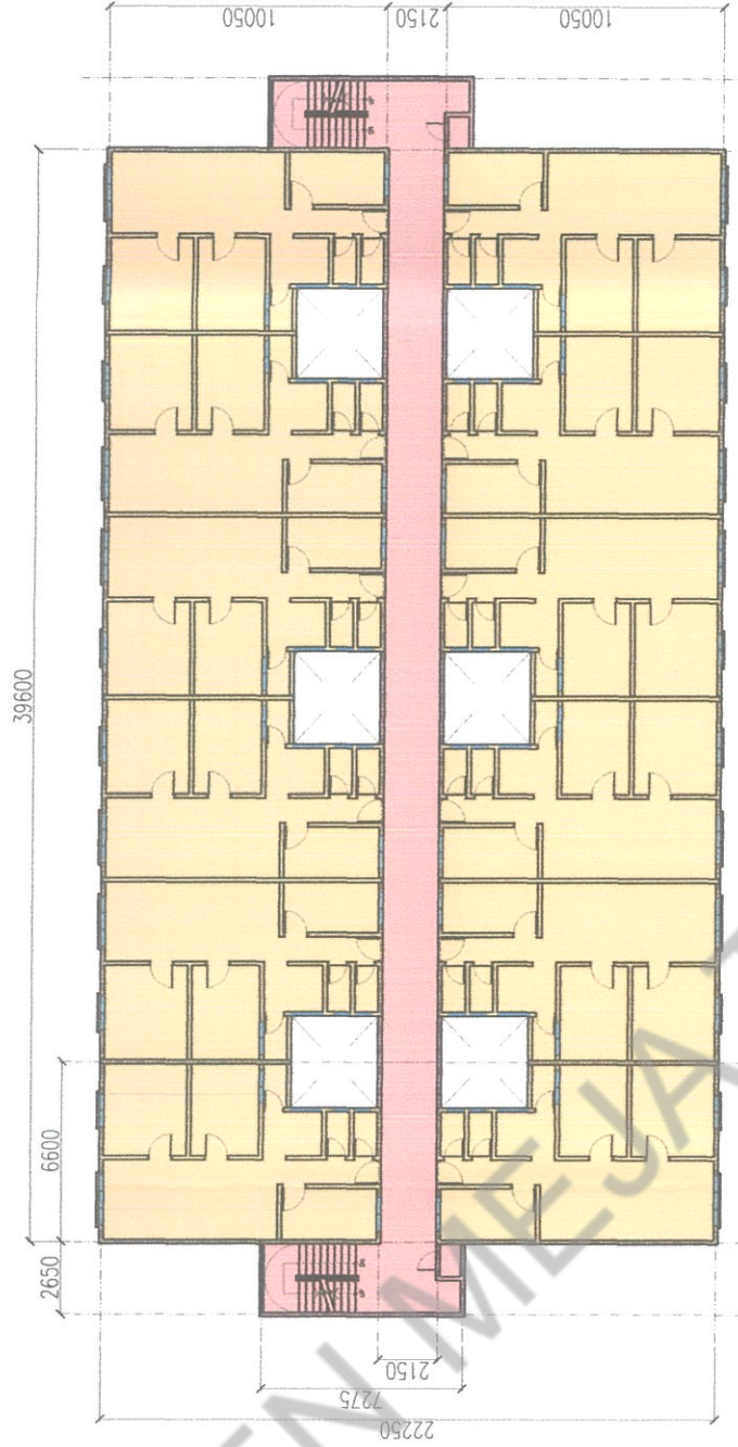
1ST. FL. TO 5TH. FL. PLAN BLOCK A SCALE : 1:300
