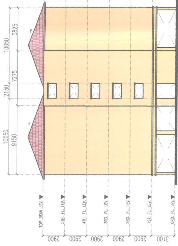
RIGHT ELEVATION BLOCK A SCALE : 1:300
